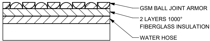
DETAIL A SCALE 1 : 1
